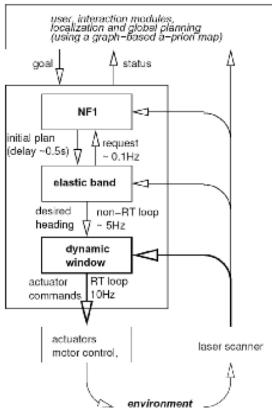
Figure 6.17 Flow diagram of the ASL approach [122].
