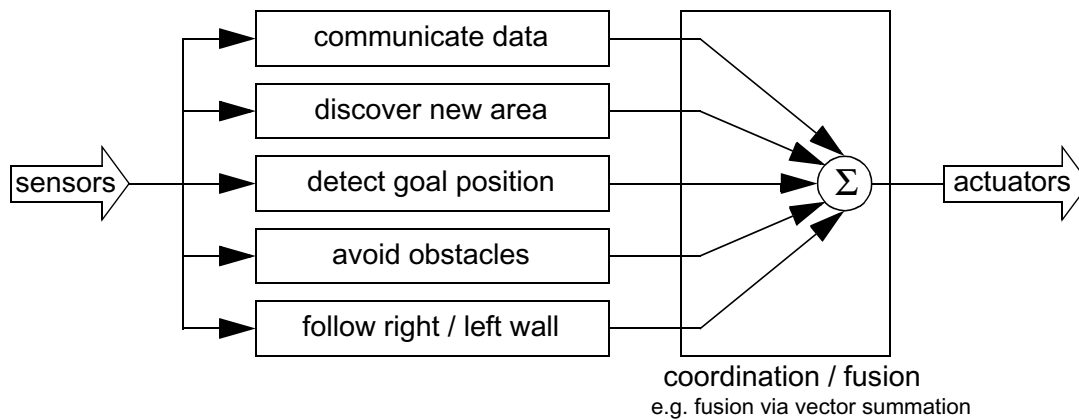
Figure 5.7 An architecture for behavior-based navigation.
