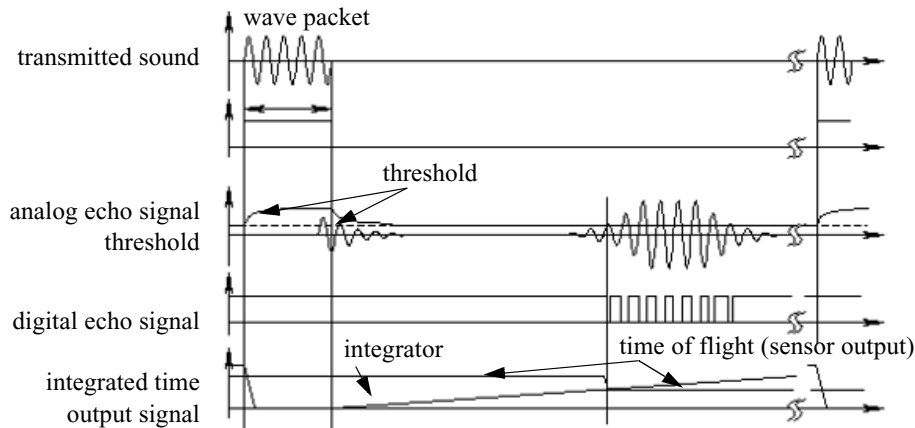
Figure 4.6 Signals of an ultrasonic sensor.
