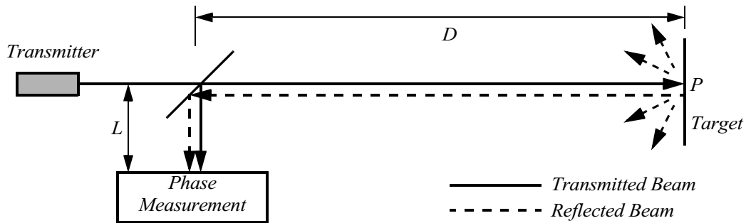
Figure 4.9 Schematic of laser rangefinding by phase-shift measurement.
