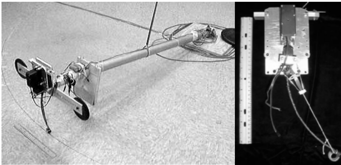
Figure 2.10 The 2D single bow leg hopper [46]. Image courtesy of H. Benjamin Brown and Garth Zeglin, CMU.
