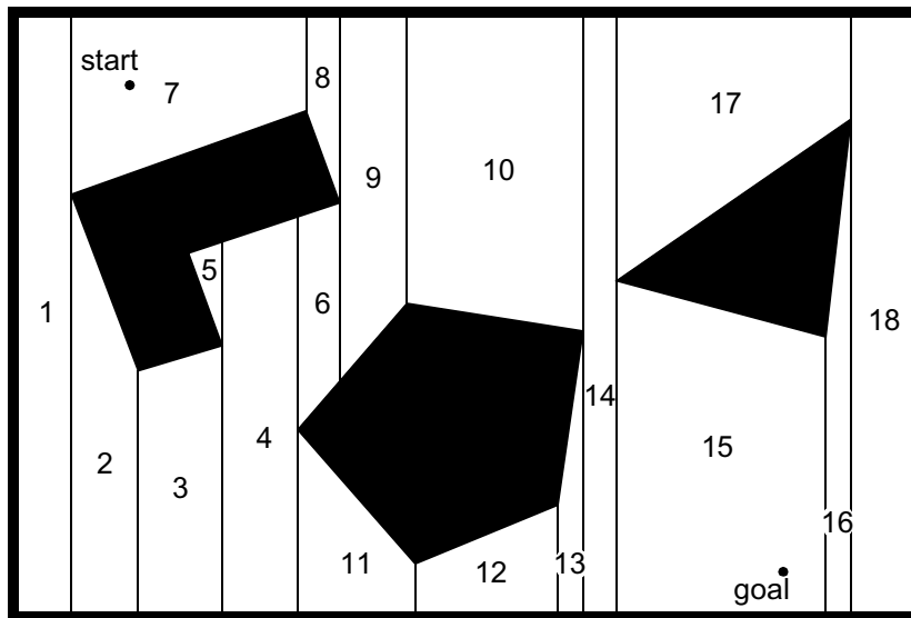
Figure 5.14 Example of exact cell decomposition.
