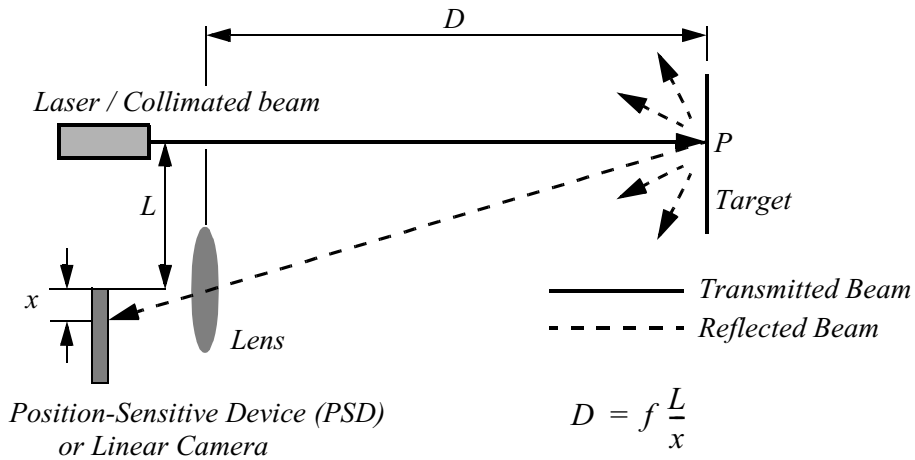
Figure 4.13 Principle of 1D laser triangulation.
