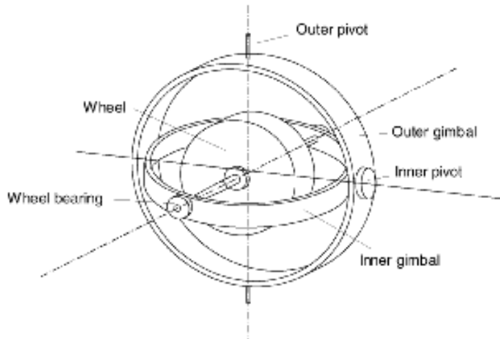
Figure 4.4 Two-axis mechanical gyroscope.
