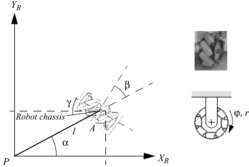
Figure 3.8 A Swedish wheel and its parameters.
