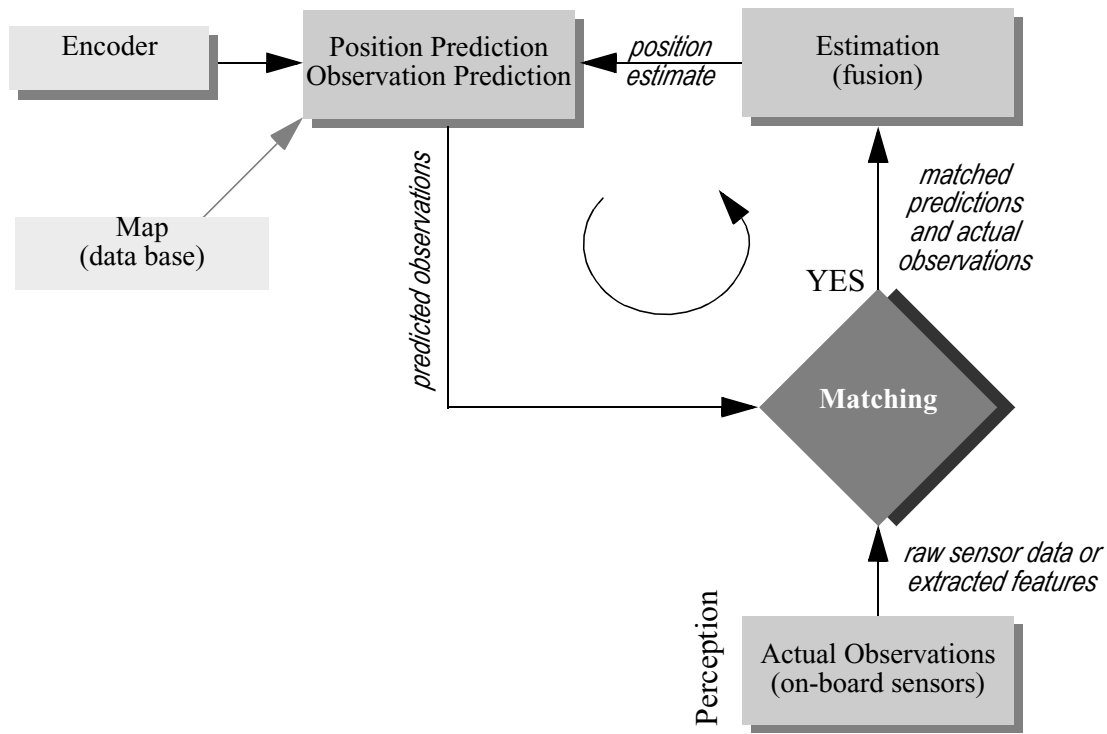
Figure 5.28 Schematic for Kalman filter mobile robot localization (see [23]).
