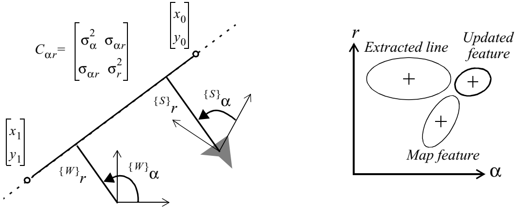
Figure 5.39 Uncertainties in the map.
