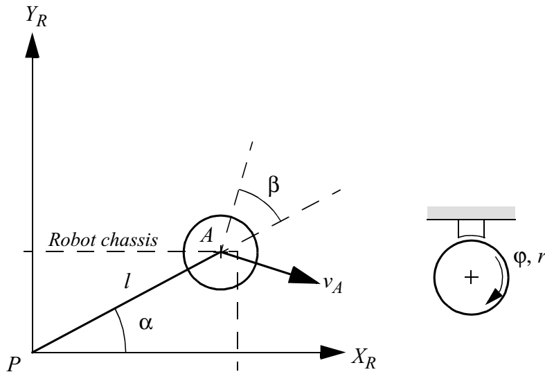
Figure 3.9 A spherical wheel and its parameters.
