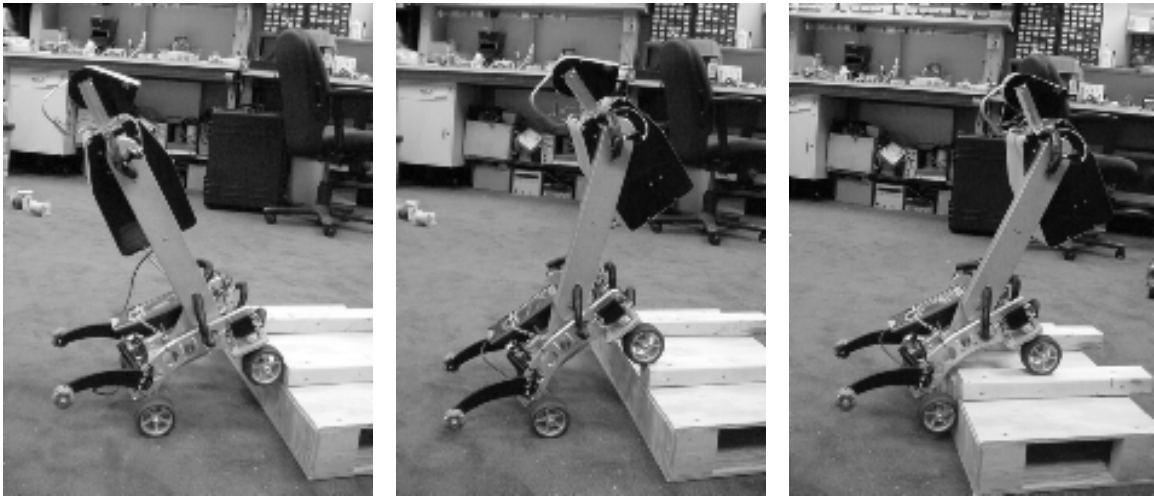
Figure 2.28 The Personal Rover, demonstrating ledge climbing using active center-of-mass shifting.
