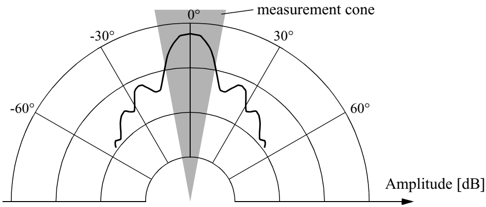
Figure 4.7 Typical intensity distribution of an ultrasonic sensor.
