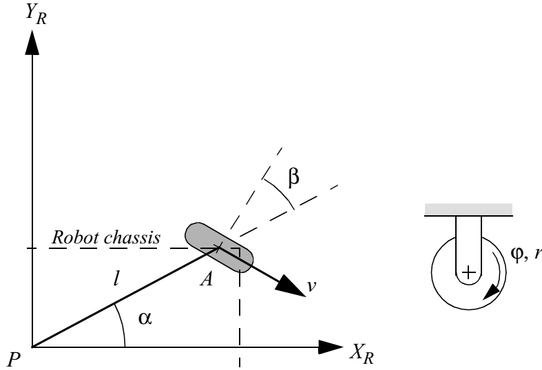
Figure 3.4 A fixed standard wheel and its parameters.
