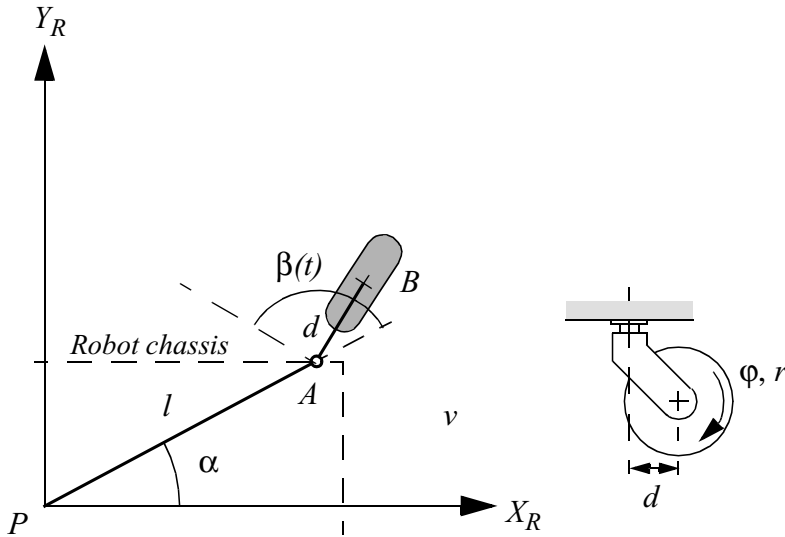
Figure 3.6 A castor wheel and its parameters.
