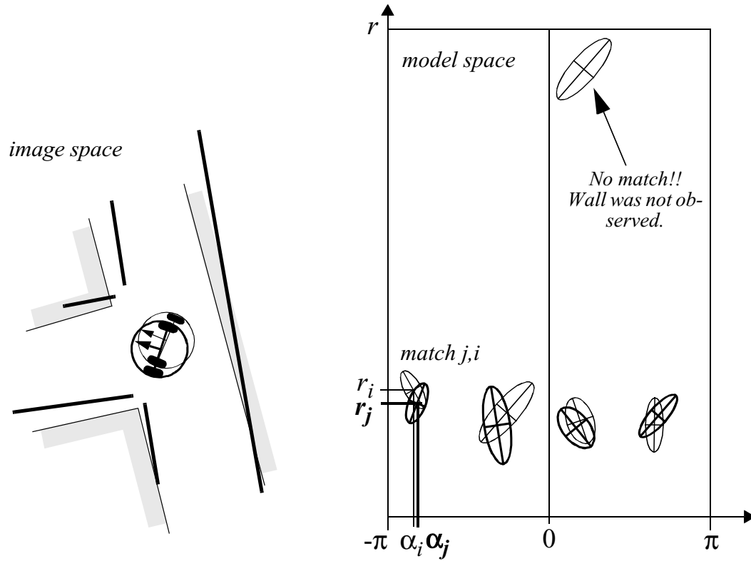
Figure 5.33 Matching: The observations (thick) and measurement prediction (thin) are matched and the innovation and its uncertainties are calculated.
