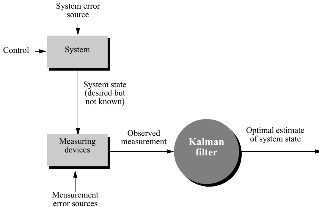
Figure 5.25 Typical Kalman filter application [106].
