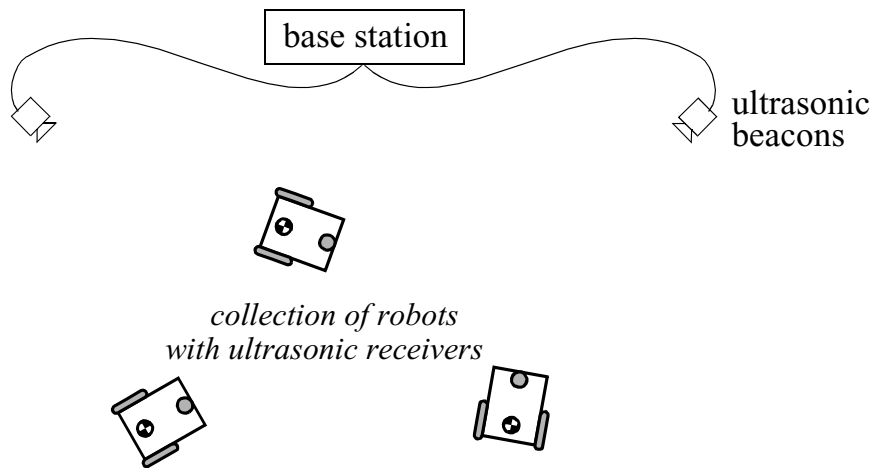
Figure 5.36 Active ultrasonic beacons.
