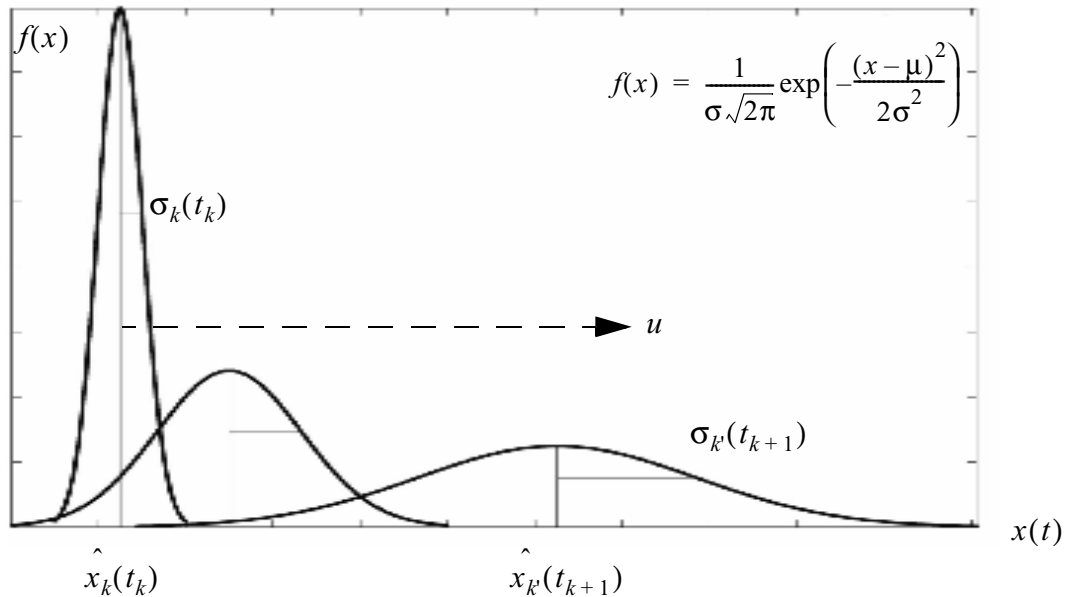
Figure 5.27 Propagation of probability density of a moving robot [106].
