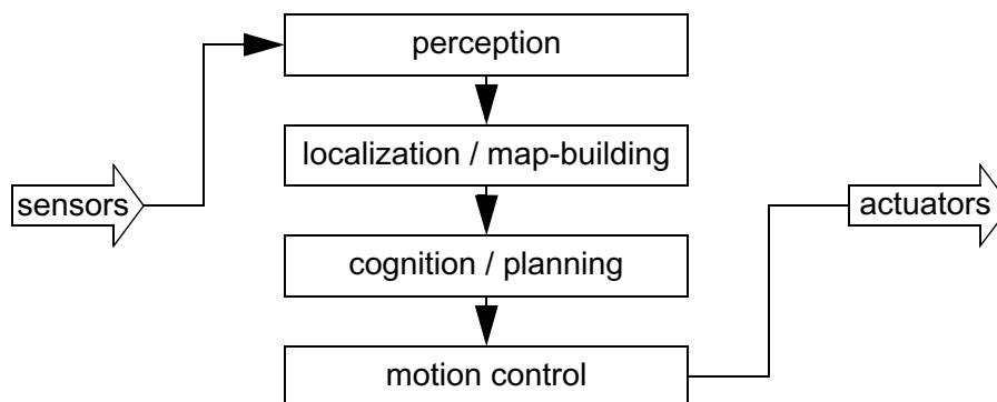
Figure 5.8 An architecture for map-based (or model-based) navigation.
