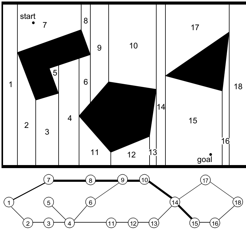
Figure 6.4 Example of exact cell decomposition.
