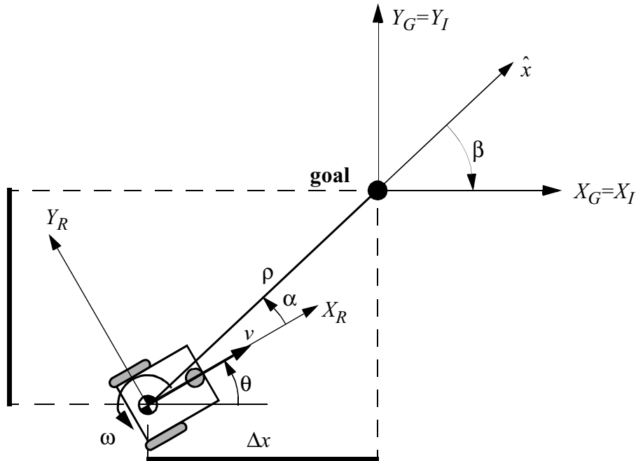
Figure 3.19 Robot kinematics and its frames of interests.
